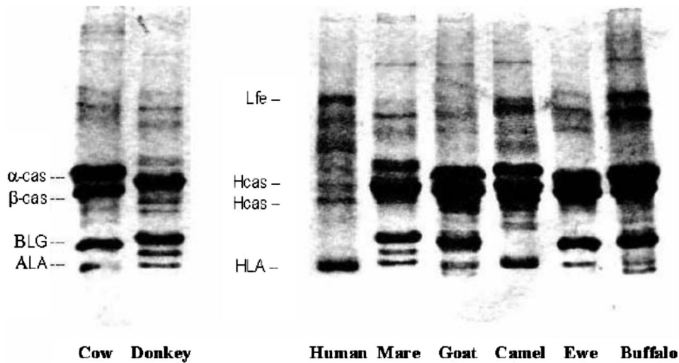
FIGURE 4-1. SDS-PAGE of mammalian milk samples. Hcas = human casein; HLA = human lactalbumin; Lfe = human lactoferrin; \alpha -cas = bovine alpha casein; \beta -cas = bovine beta casein; BLG = bovine \beta -lactoglobulin; ALA = bovine \alpha -lactalbumin.
